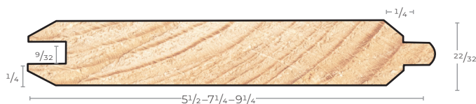
CENTRE 'V' MATCH 2S
