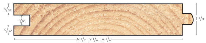
5/4 CENTRE MATCHED N° 14C
