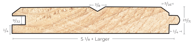
CENTRE 'V' MATCH 1S WIDE 'V'
