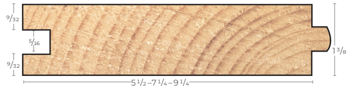
5/4 CENTRE MATCHED N° 14C
